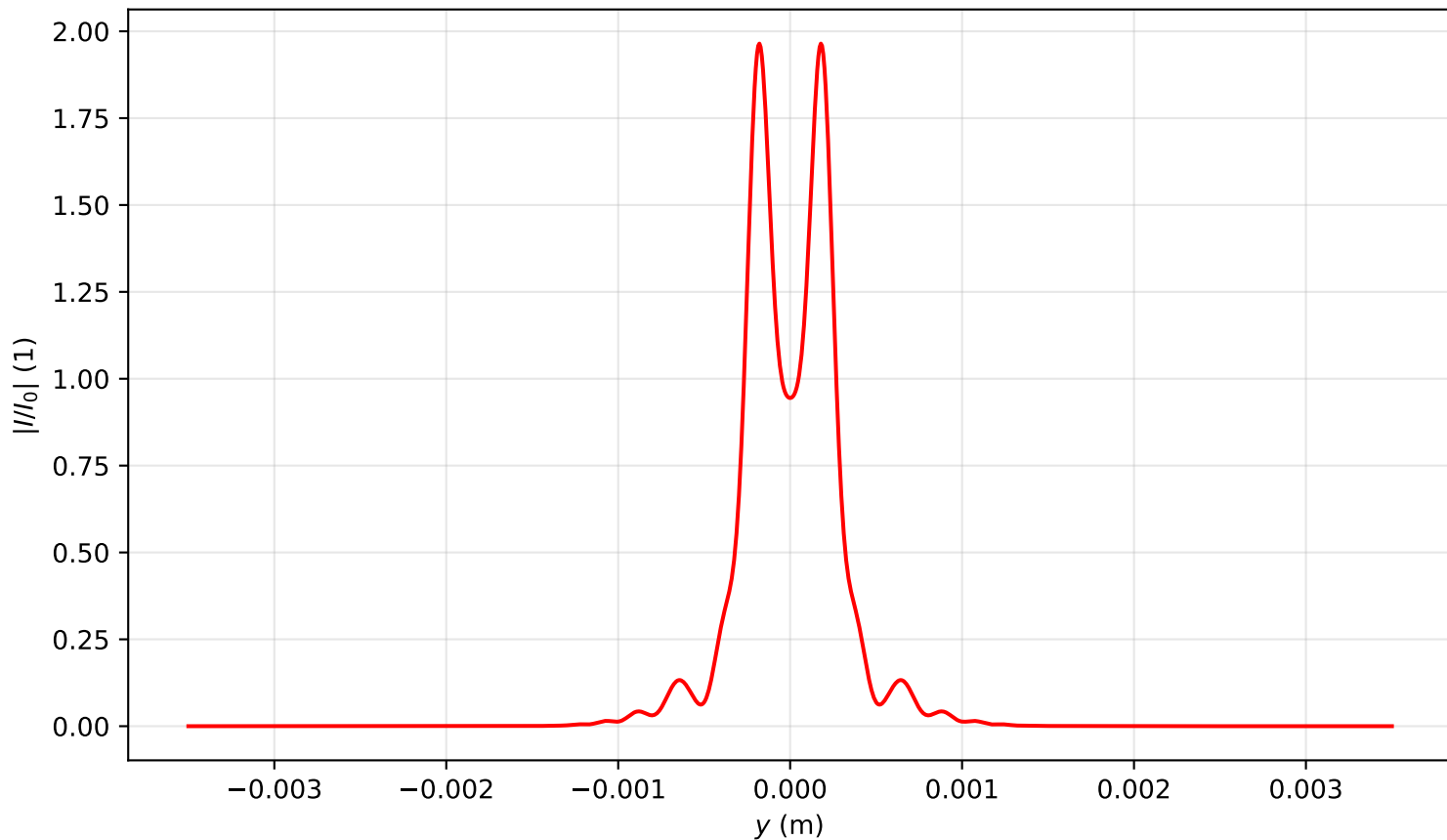
Intensity profile I(x=0, y, z=0.955)/I_0 , P_{in}=3.0P_{cr} , artificial time
